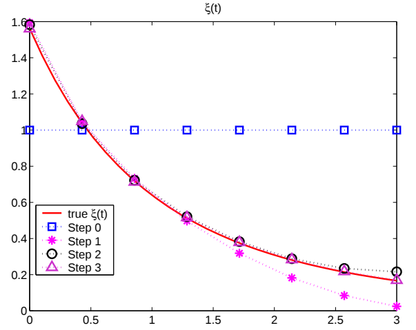
Figure 6: \xi^{(0)}(t) = 1 , N = 8
