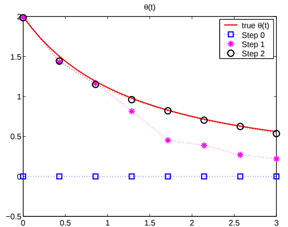
Figure 2: \theta^{(0)}(t) = 0 , N = 8
