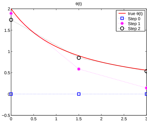
Figure 1: \theta^{(0)}(t) = 0 , N = 3
