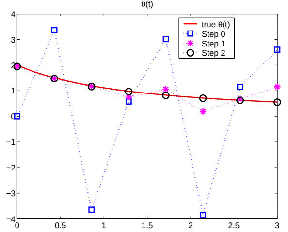
Figure 4: \theta^{(0)}(t) = P^8(4 \sin 5t) , N = 8
