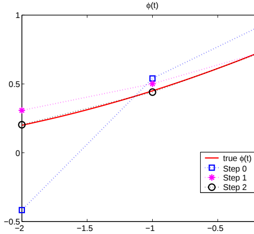
Figure 7: \varphi^{(0)}(t) = P^3(\cos t) , N = 3
