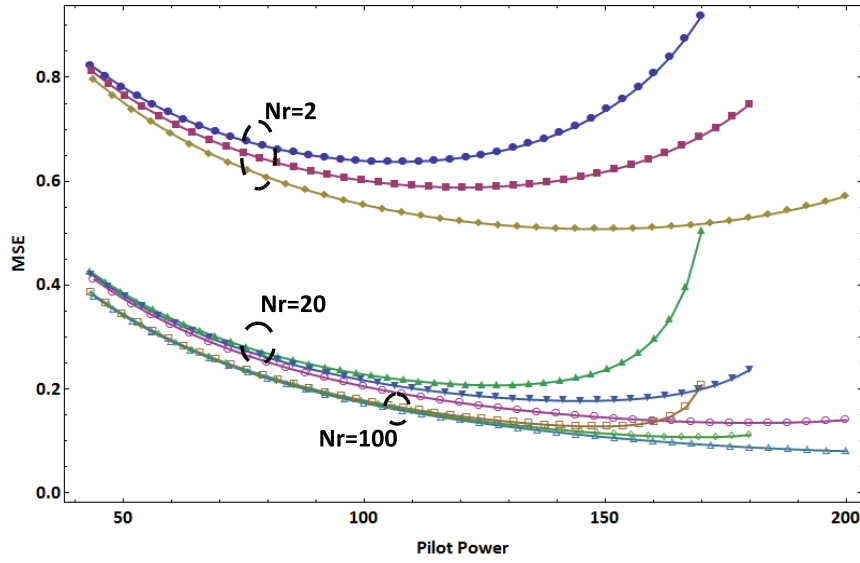
Fig. 3.4 The MSE as a function of the pilot power of a SIMO system with N_r = 2, 20, 100 antennas respectively, for 3 different sum power constraints (200 mW, 225 mW and 250 mW). As the number of antennas increases, the optimal pilot power increases.
