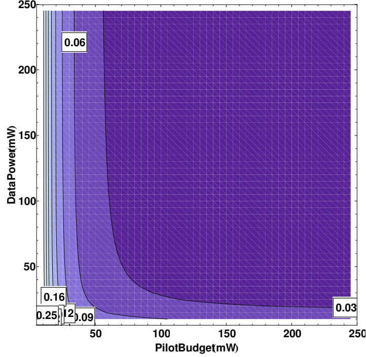
Fig. 5.1 Contour plot of the MSE achieved by specific pilot and data power settings of a SIMO system with N_r = 20 uncorrelated receiver antennas at a fix path loss position of 50 dB. For example an MSE value less than 0.03 can be reached by setting the pilot power budget to \tau_p P_p \geq 70 mW and the data power P \geq 60 mW, or by P_p \geq 200 mW and P \geq 20 mW. We can see that with a total power budget of 250 mW, and with proper pilot-data balancing, a minimum MSE that is clearly less than 0.03 can be reached.
